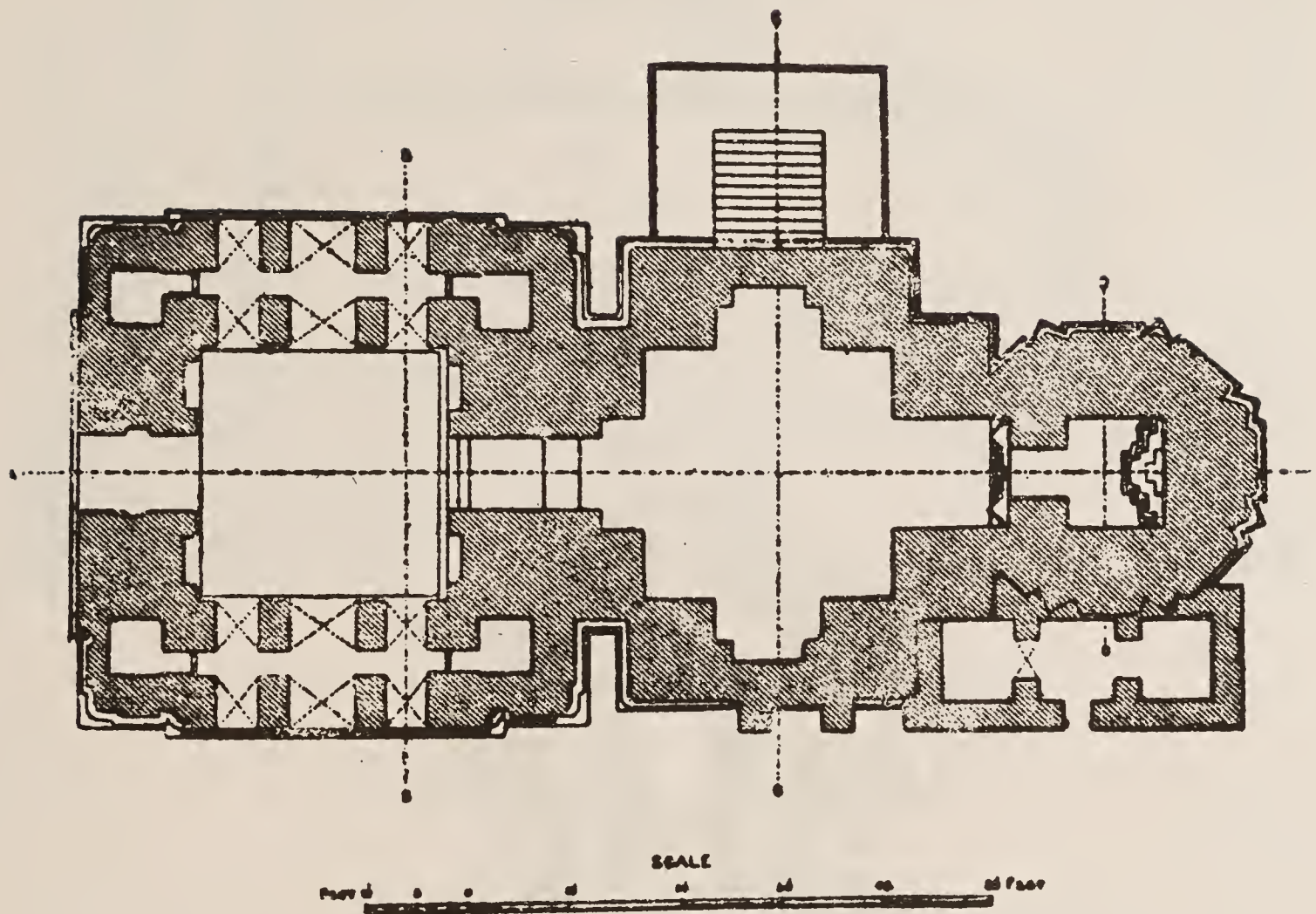
Fig. 3 Nurpur Fort, Temple: Plan
