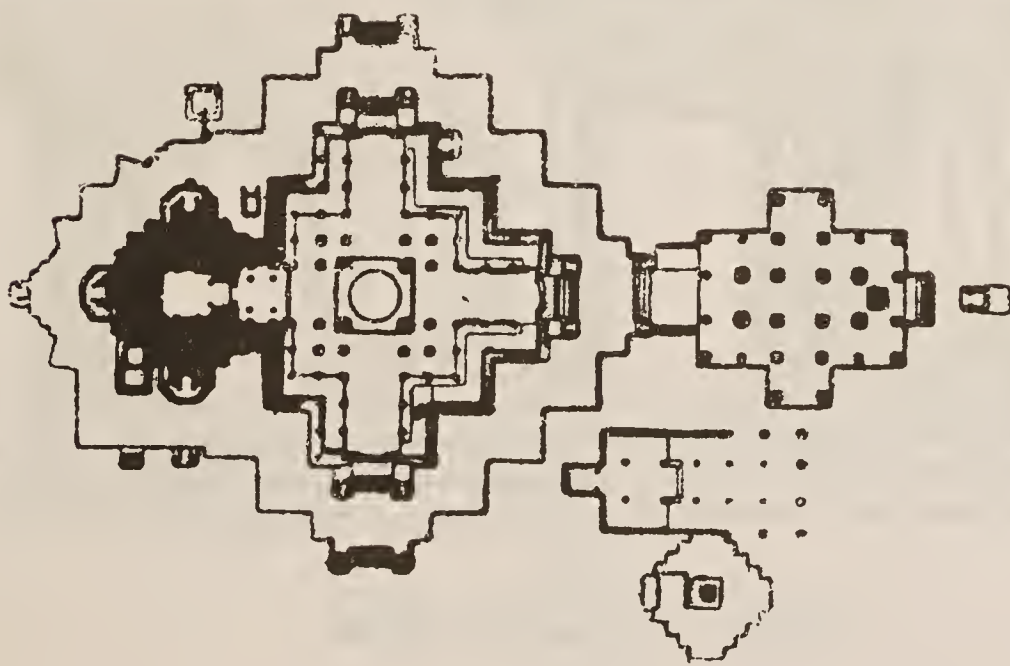
Fig. 52 Belur, Chenna Kesava temple: Plan
