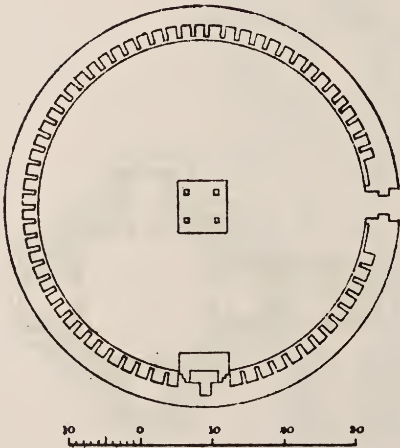
Fig. 10 Rānīpur Jhariāl, Circular Yoginī temple: Plan
