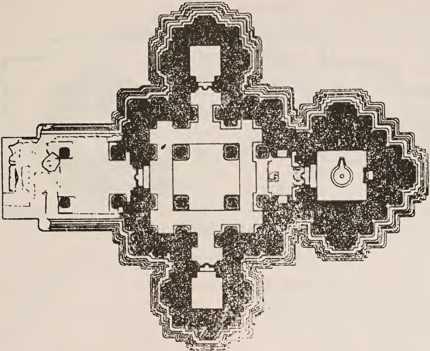
Fig. 27 Balsane: Temple No. 1: Plan
