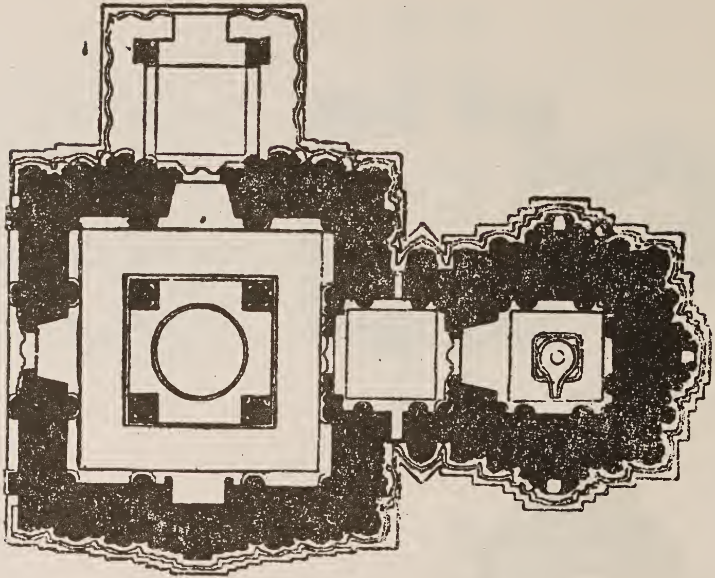
Fig. 49 Gadag, Someśvara temple: Plan
