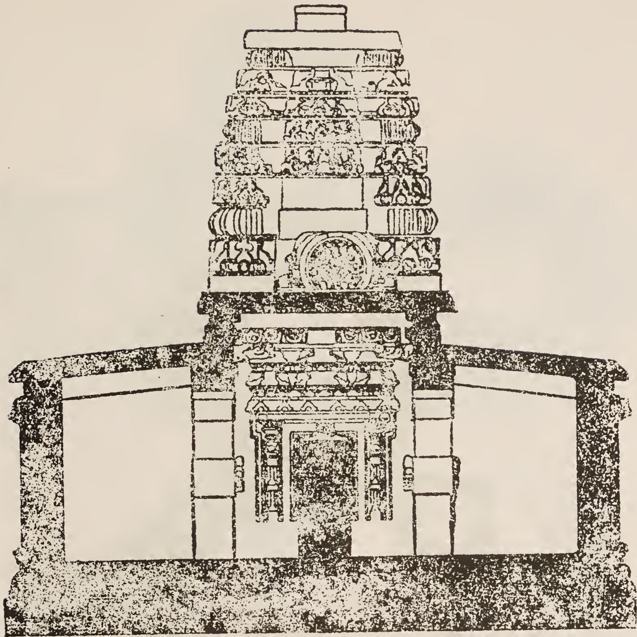
Fig. 24 Aihole, Temple No 9: Elevation
