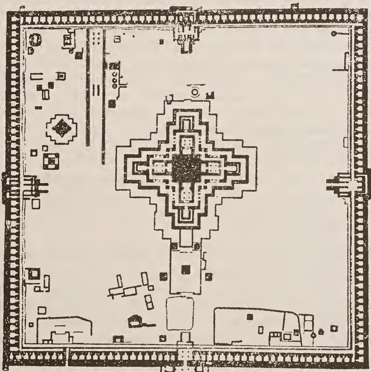
Fig. 57 Pāhārpur, Great temple: Plan
