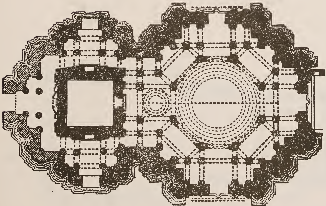
Fig. 22 Somanāthapattana: Somanātha temple: Plan
