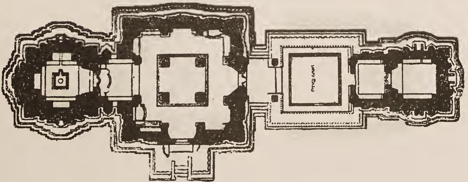
Fig. 45 Lakkundi, Kāśīveśvara temple: Plan
