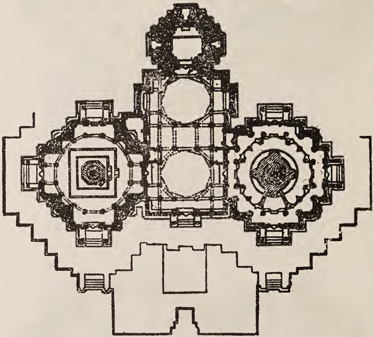
Fig. 23 Girnar, Triple-shrined temple: Plan
