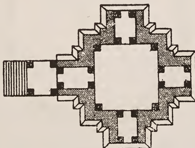
Fig. 8 Khajurāho, Mritang Mahādeo Temple: Plan
