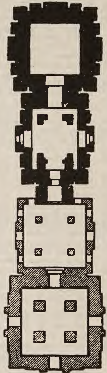
Fig. 2 Bhuvaneśvara, Liṅgarāja Temple: Plan
