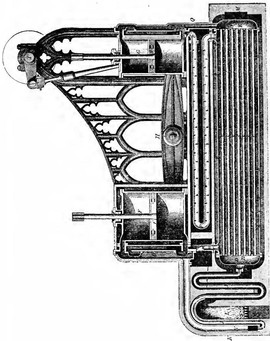
Ericsson's Caloric Engine.
