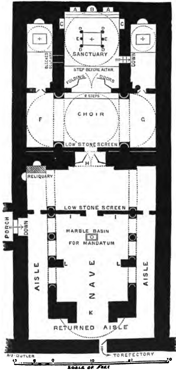
ILL. 62. — Plan of Dair-as-Suriâni. (From Butler)
