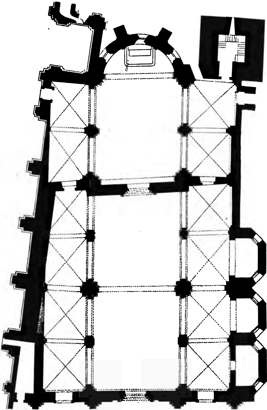
ILL. 102. — Plan of S. Celso, Milan. (From Dartein)
