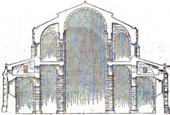
ILL. 180. — Section of St. Sernin of Toulouse. (From Dehio)
