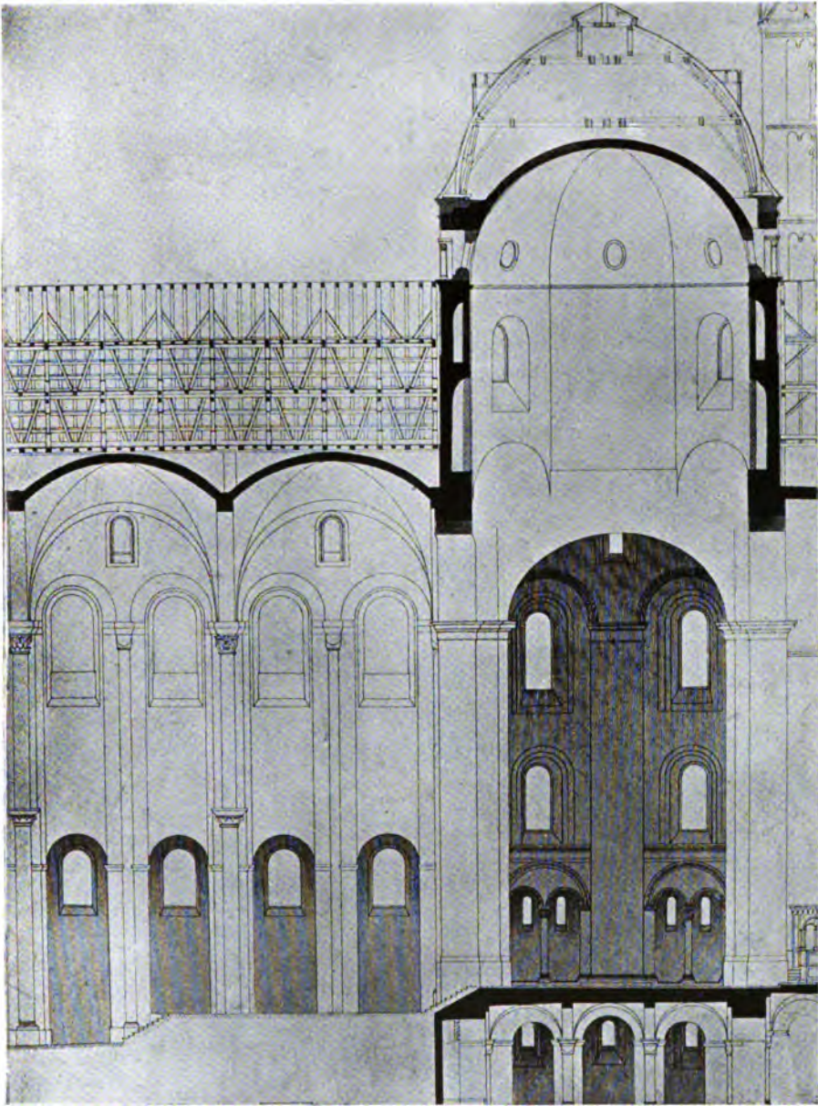
ILL. 153. — Section of Dom, Speyer. (From Meyer-Schwartau)
