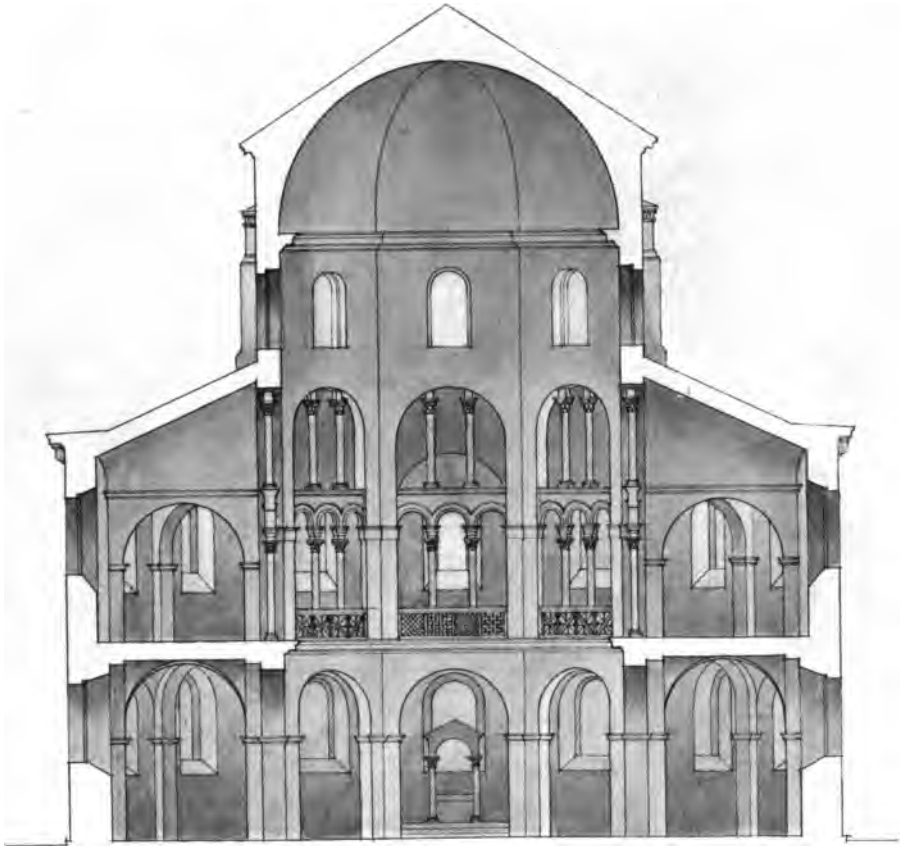
ILL. 86. — Section of Dom at Aachen
