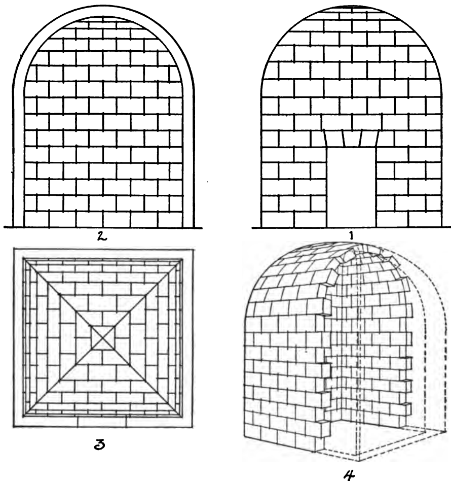
ILL. 11. — The Cloistered Vault, Diagram
