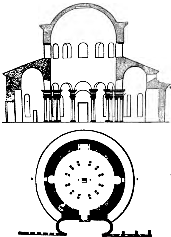
ILL. 44. — Plan and Section of Sta. Costanza, Rome. (From Canina)
