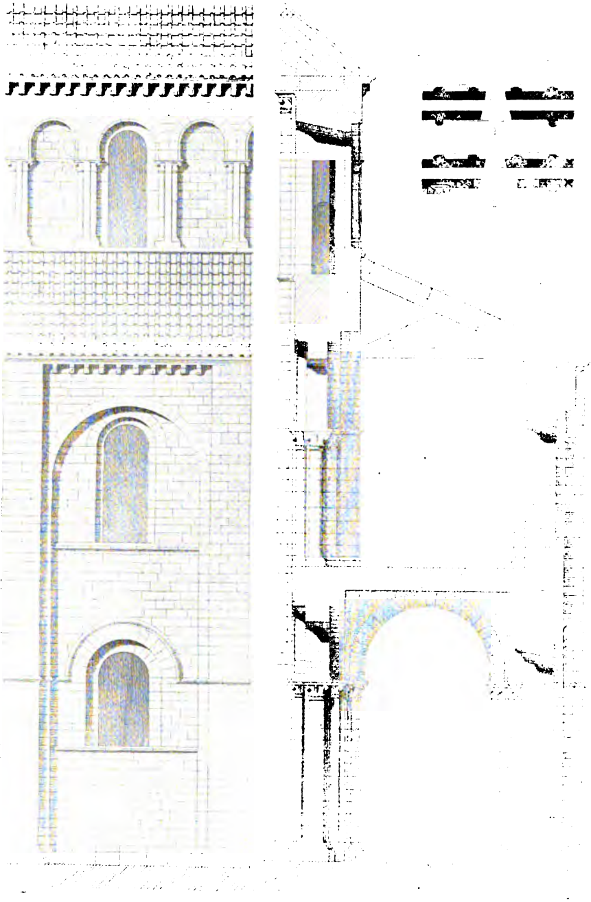
ILL. 126. — Abbaye-aux-Hommes, Caen. Exterior Elevation and Section Restored by Ruprich-Robert
